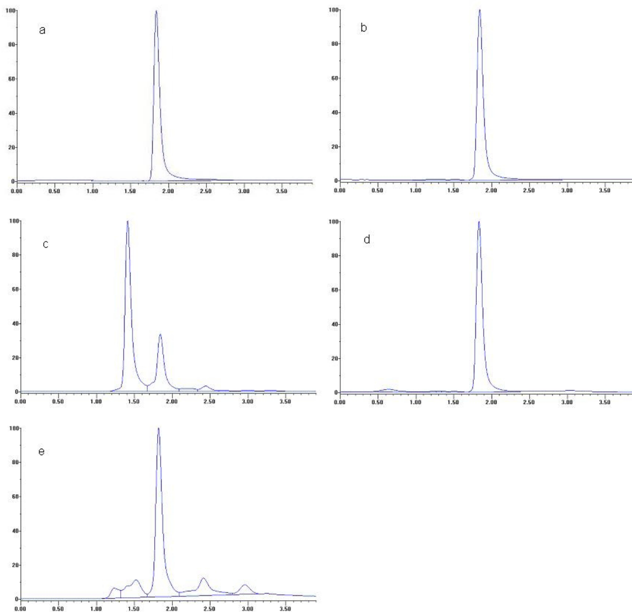
Figure 1. Representative chromatograms of FEN standard (a), neutral hydrolysis (b), chemical oxidation (c) acid hydrolysis (d) and alkaline hydrolysis (e). Concentration: 0.075 mg.mL -1 . Chromatographic conditions: Thermo C 18 column (150 x 3.9 mm, 5 µm); mobile phase: acetonitrile:water (30:70, v/v) with 0,1% triethylamine and pH adjusted to 5.0 with formic acid; flow rate, 1.0 mL.min -1 , UV detection at 276 nm and temperature of 20 ± 1 °C
